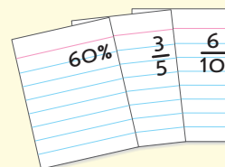
Scoring Set
