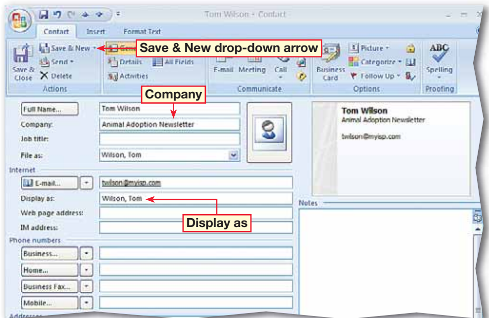
FIGURE 2.3 New contact
