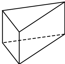
triangular prism
