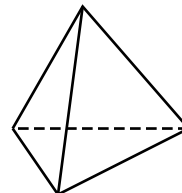
triangular pyramid
